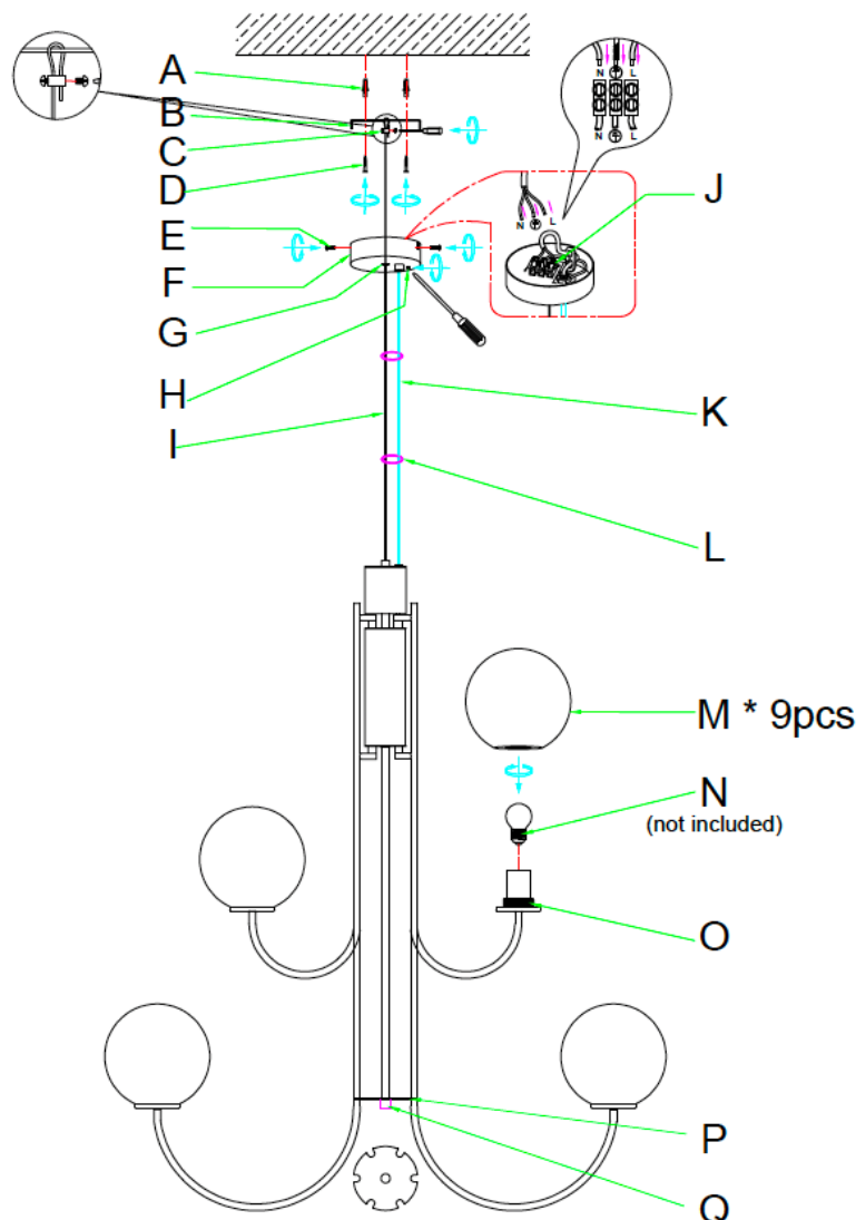
Fig. 2 Installation Diagram
